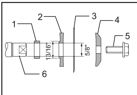
► 1. Ring 17 2. Inner flange 3. Blade 4. Outer flange 5. Hex bolt 6. Mounting shaft
